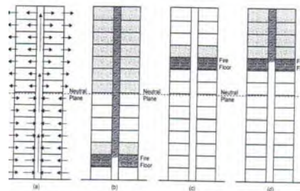
Air and smoke movement in a high-rise building due to stack effect: (a) airflow due to stack effect, (b) fire below the neutral plane, (c) fire above the neutral plane, and (d) fire above the neutral plane with smoke entering a shaft due to buoyancy.
